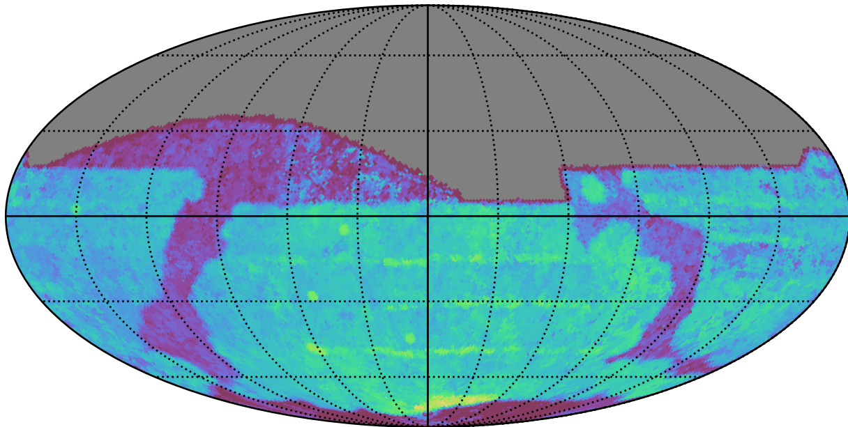
ddf_loaded_fl2_v3.4_10yrs All sky z band: Median Season Length
