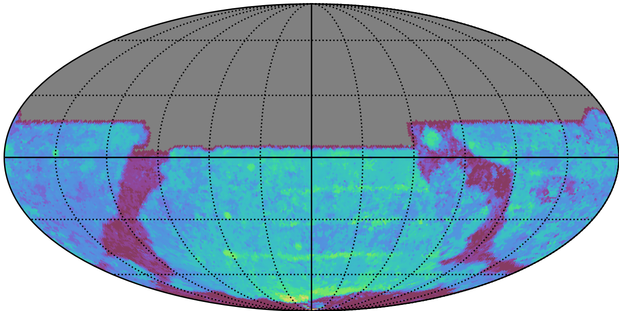
ddf_loaded_fl2_v3.4_10yrs All sky y band: Median Season Length
