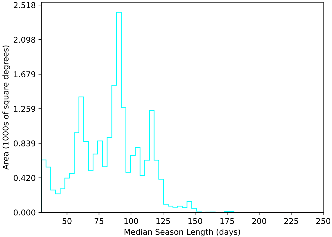
ddf_loaded_fl2_v3.4_10yrs All sky u band: Median Season Length
