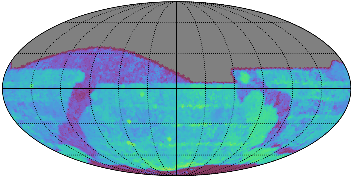
ddf_loaded_fl2_v3.4_10yrs All sky r band: Median Season Length
