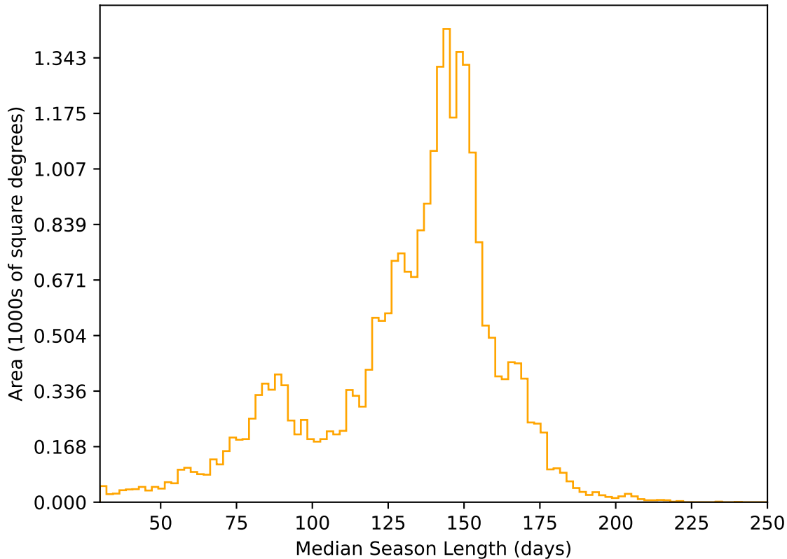
ddf_loaded_fl2_v3.4_10yrs All sky r band: Median Season Length
