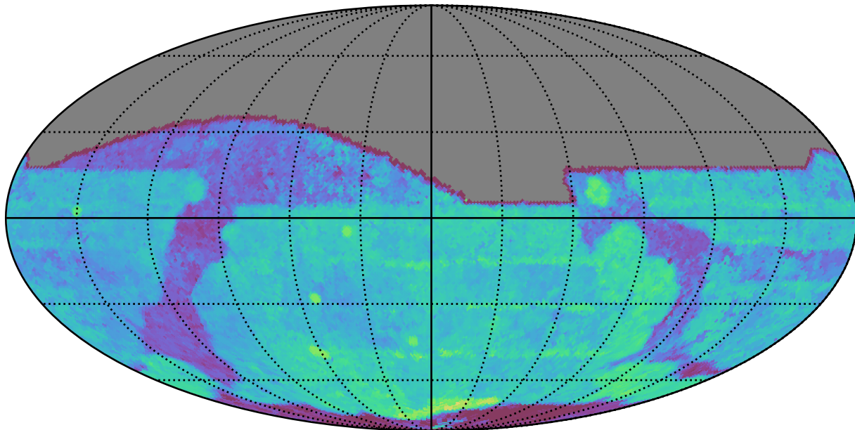
ddf_loaded_fl2_v3.4_10yrs All sky i band: Median Season Length
