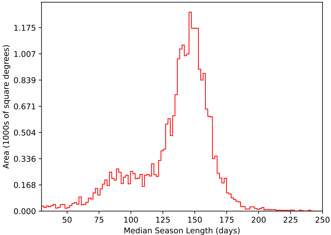
ddf_loaded_fl2_v3.4_10yrs All sky i band: Median Season Length
