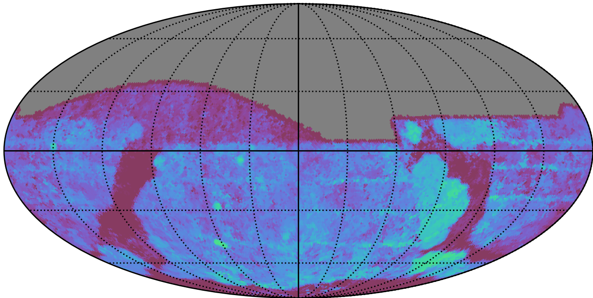
ddf_loaded_fl2_v3.4_10yrs All sky g band: Median Season Length
