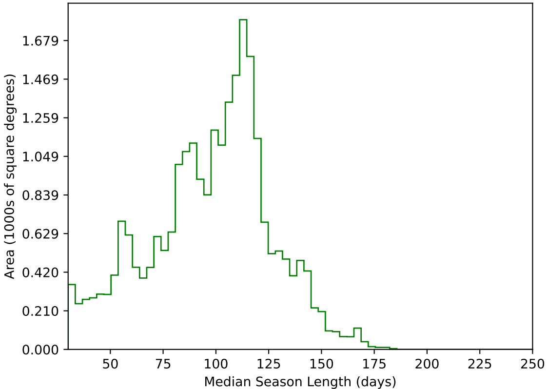
ddf_loaded_fl2_v3.4_10yrs All sky g band: Median Season Length
