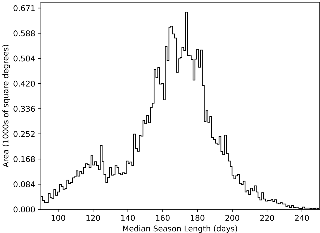
ddf_loaded_fl2_v3.4_10yrs All sky all bands: Median Season Length
