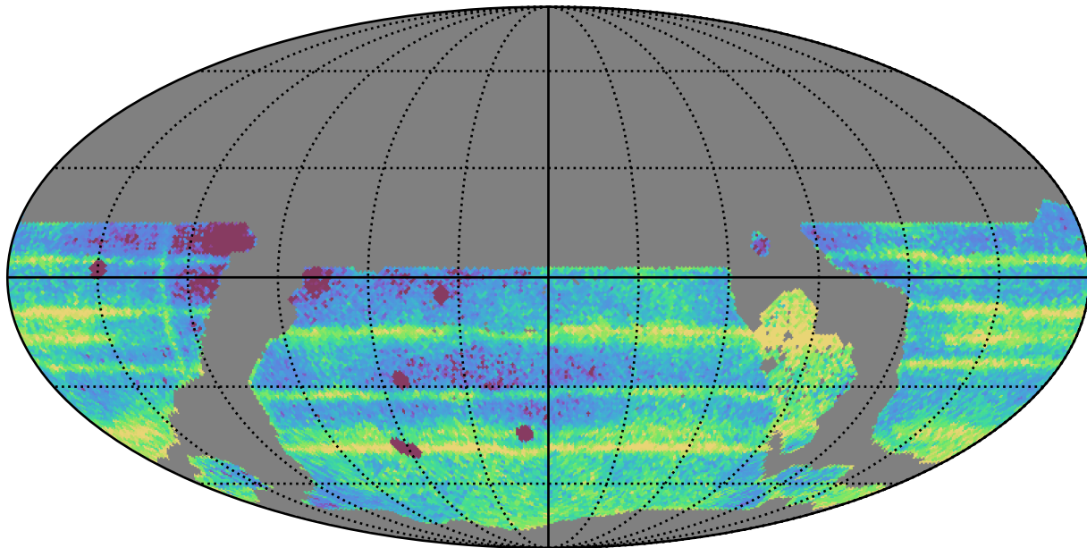
ddf_loaded_fl2_v3.4_10yrs WFD: Median Intra-Night Gap
