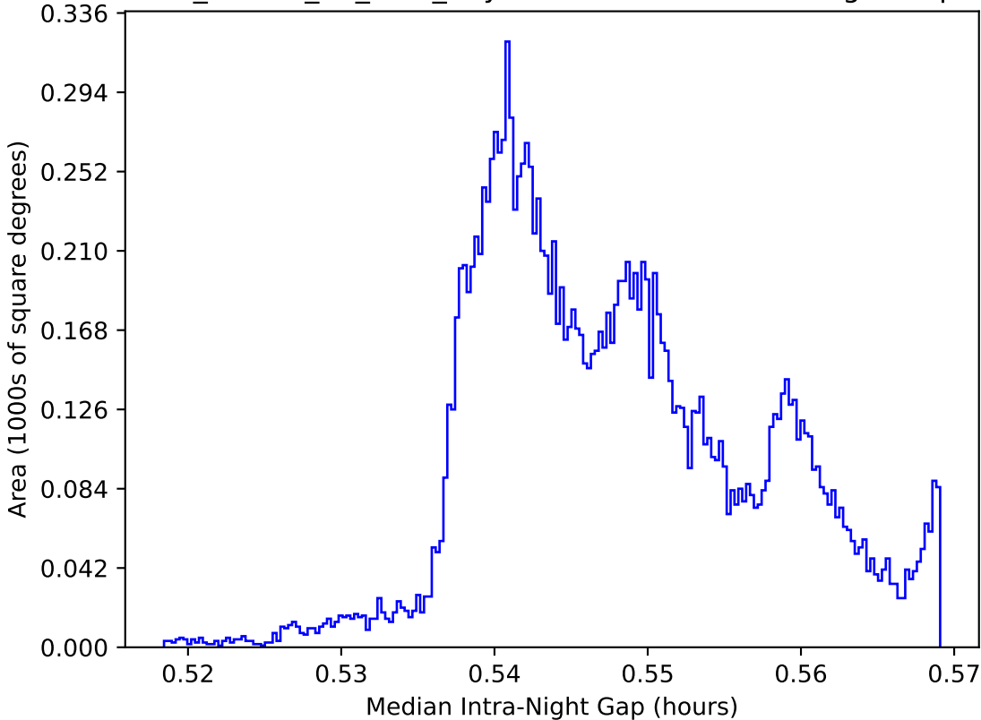
ddf_loaded_fl2_v3.4_10yrs WFD: Median Intra-Night Gap
