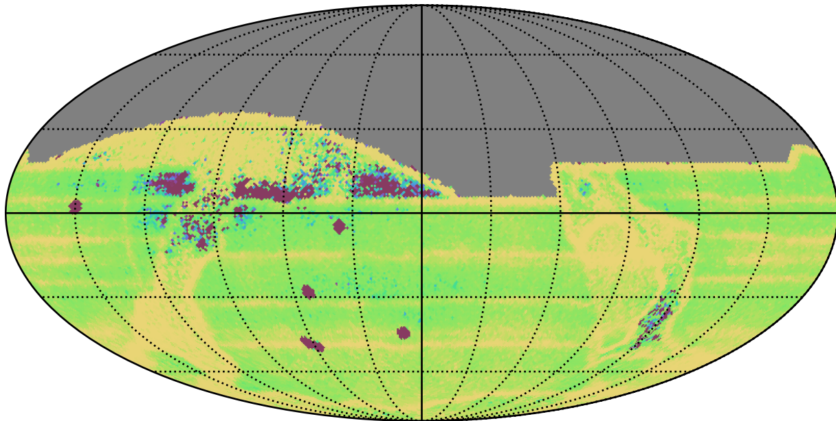
ddf_loaded_fl2_v3.4_10yrs All sky: Median Intra-Night Gap
