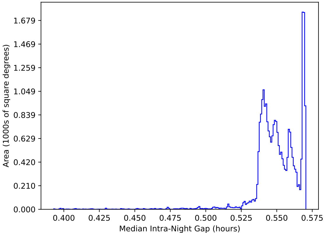
ddf_loaded_fl2_v3.4_10yrs All sky: Median Intra-Night Gap
