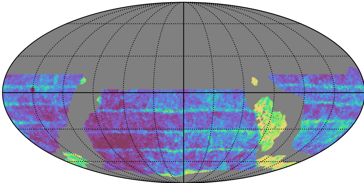
ddf_loaded_fl2_v3.4_10yrs WFD z band: Median Inter-Night Gap
