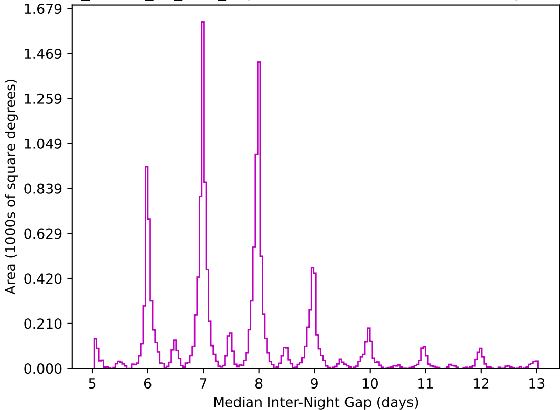
ddf_loaded_fl2_v3.4_10yrs WFD z band: Median Inter-Night Gap
