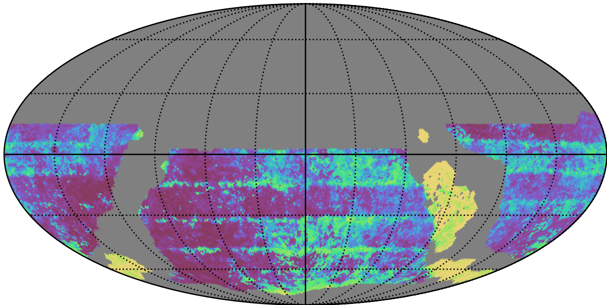
ddf_loaded_fl2_v3.4_10yrs WFD y band: Median Inter-Night Gap
