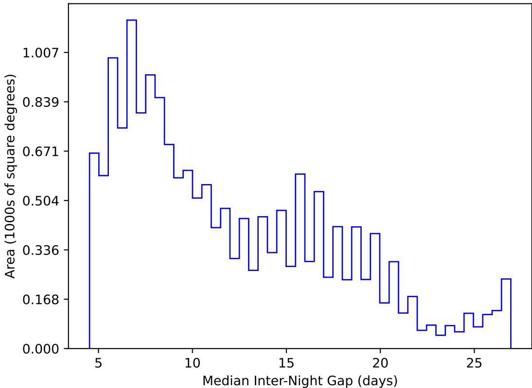
ddf_loaded_fl2_v3.4_10yrs WFD y band: Median Inter-Night Gap
