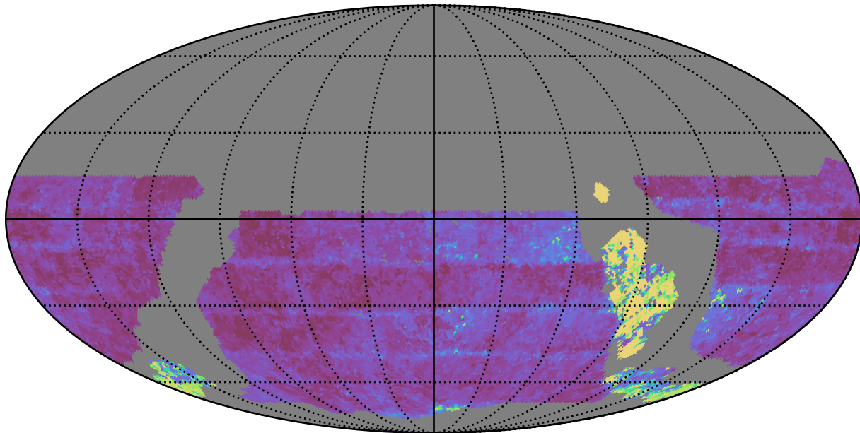
ddf_loaded_fl2_v3.4_10yrs WFD u band: Median Inter-Night Gap
