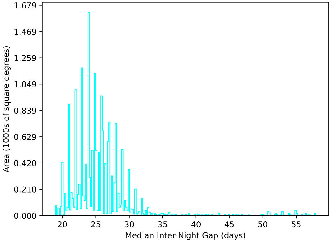
ddf_loaded_fl2_v3.4_10yrs WFD u band: Median Inter-Night Gap
