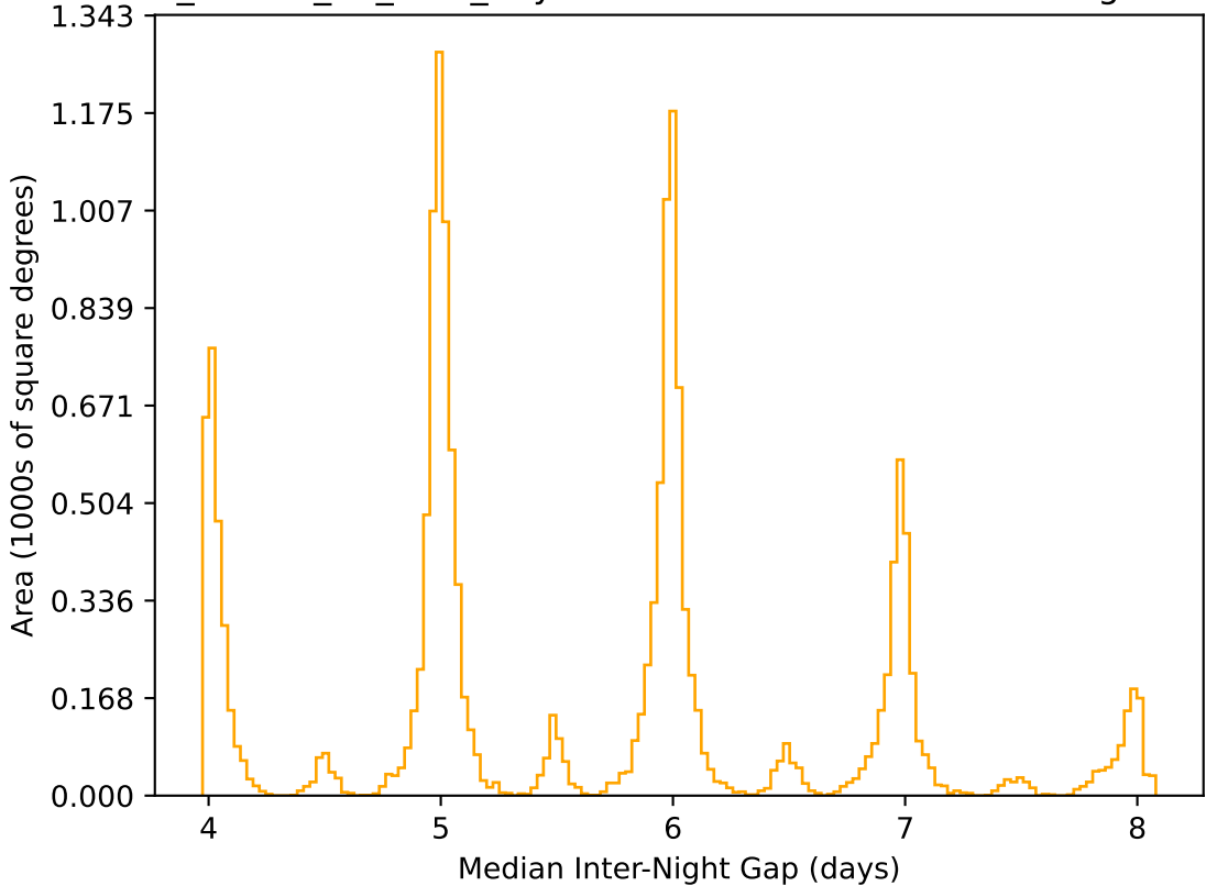
ddf_loaded_fl2_v3.4_10yrs WFD r band: Median Inter-Night Gap
