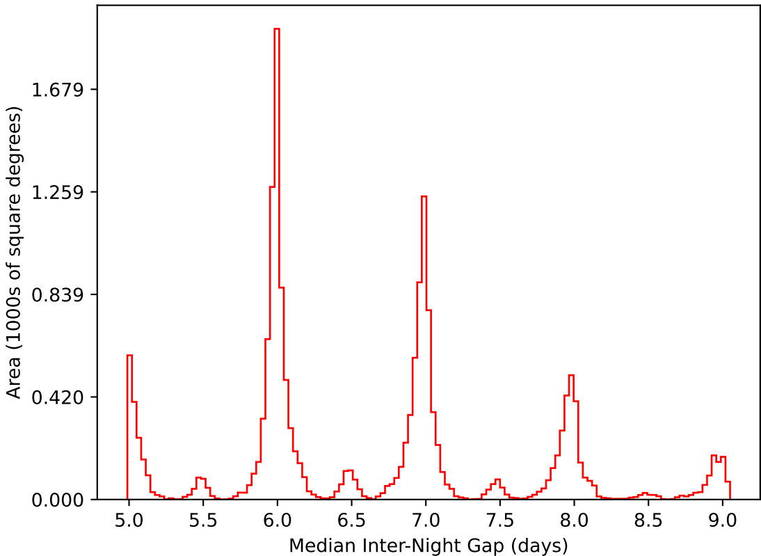
ddf_loaded_fl2_v3.4_10yrs WFD i band: Median Inter-Night Gap
