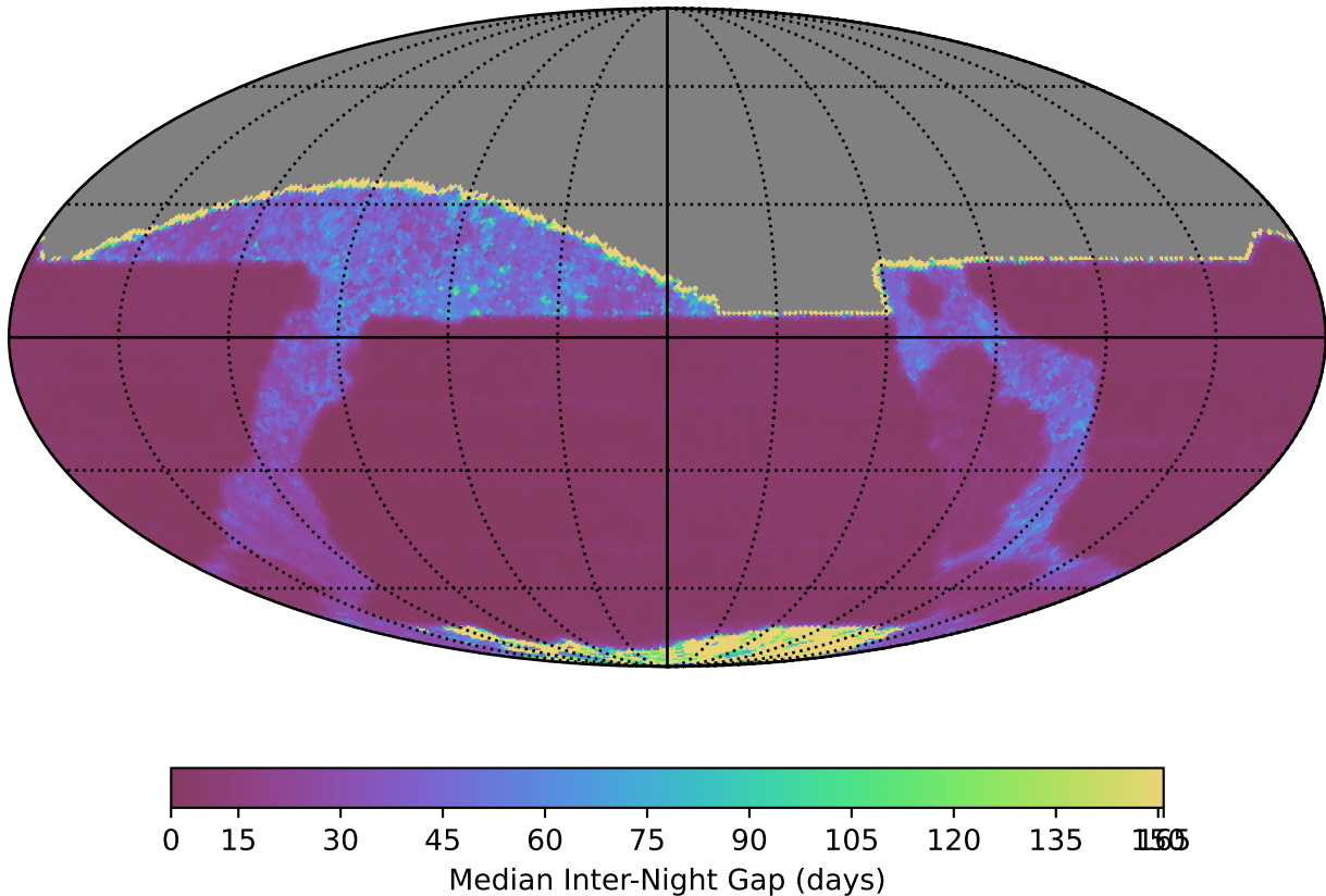
ddf_loaded_fl2_v3.4_10yrs All sky z band: Median Inter-Night Gap
