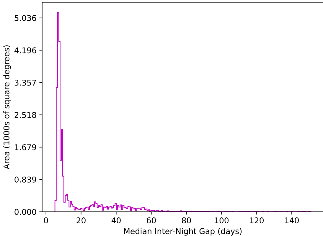
ddf_loaded_fl2_v3.4_10yrs All sky z band: Median Inter-Night Gap
