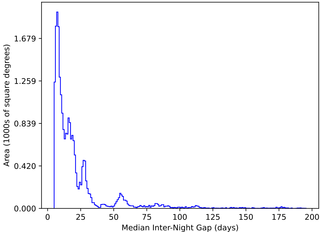
ddf_loaded_fl2_v3.4_10yrs All sky y band: Median Inter-Night Gap
