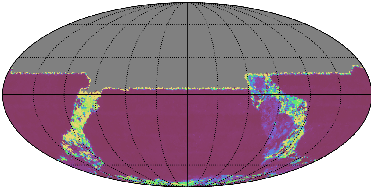
ddf_loaded_fl2_v3.4_10yrs All sky u band: Median Inter-Night Gap
