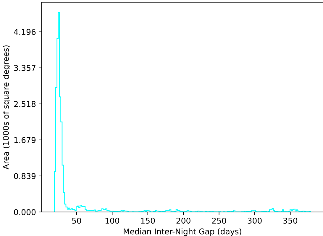
ddf_loaded_fl2_v3.4_10yrs All sky u band: Median Inter-Night Gap
