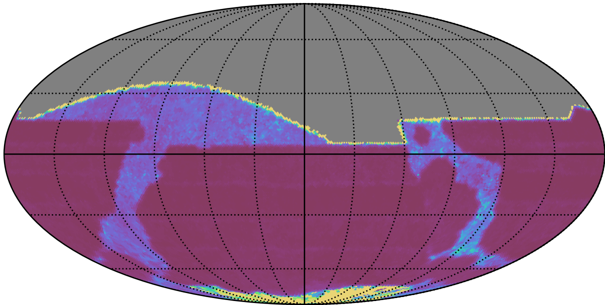
ddf_loaded_fl2_v3.4_10yrs All sky r band: Median Inter-Night Gap
