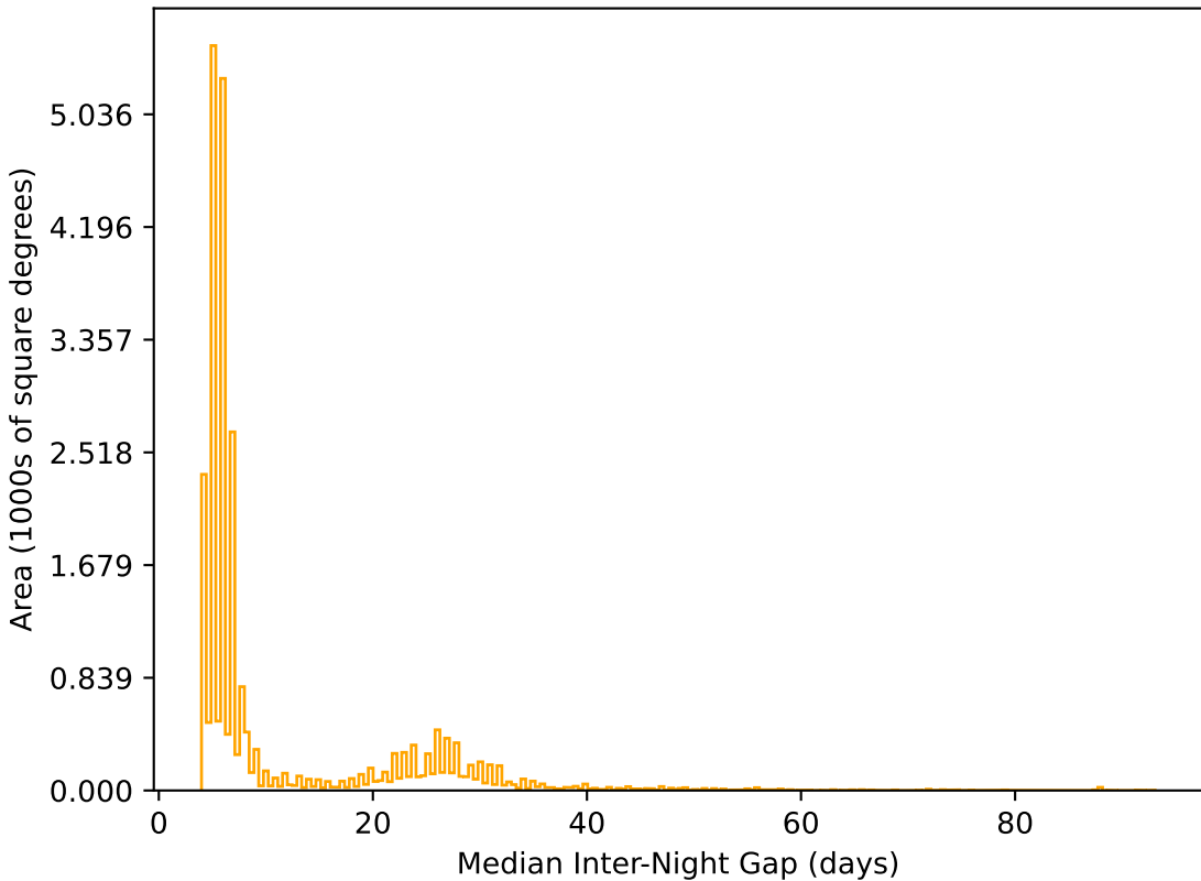
ddf_loaded_fl2_v3.4_10yrs All sky r band: Median Inter-Night Gap
