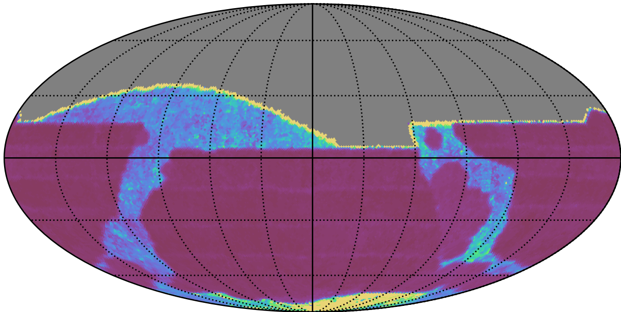
ddf_loaded_fl2_v3.4_10yrs All sky i band: Median Inter-Night Gap
