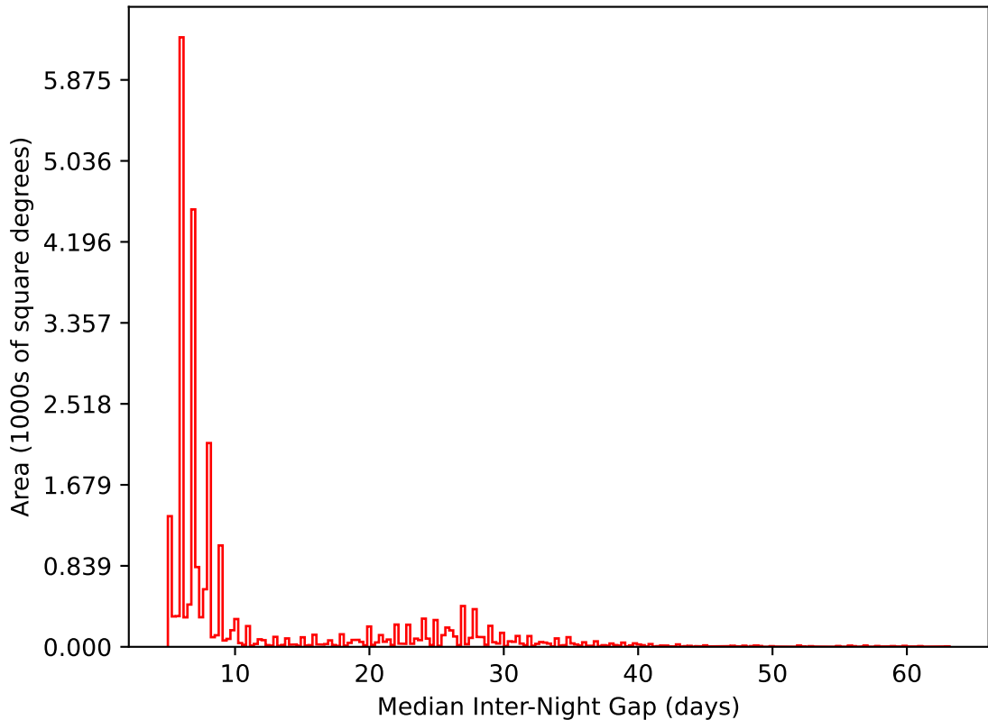
ddf_loaded_fl2_v3.4_10yrs All sky i band: Median Inter-Night Gap
