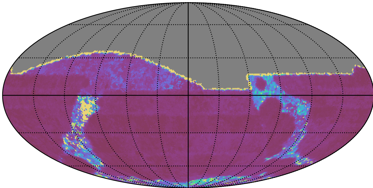
ddf_loaded_fl2_v3.4_10yrs All sky g band: Median Inter-Night Gap
