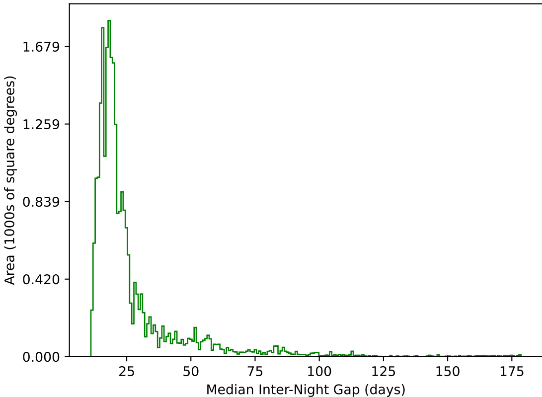
ddf_loaded_fl2_v3.4_10yrs All sky g band: Median Inter-Night Gap
