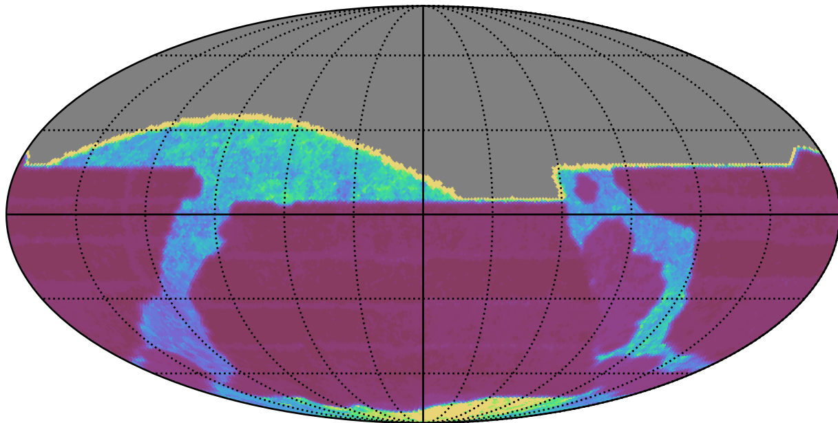
ddf_loaded_fl2_v3.4_10yrs All sky all bands: Median Inter-Night Gap
