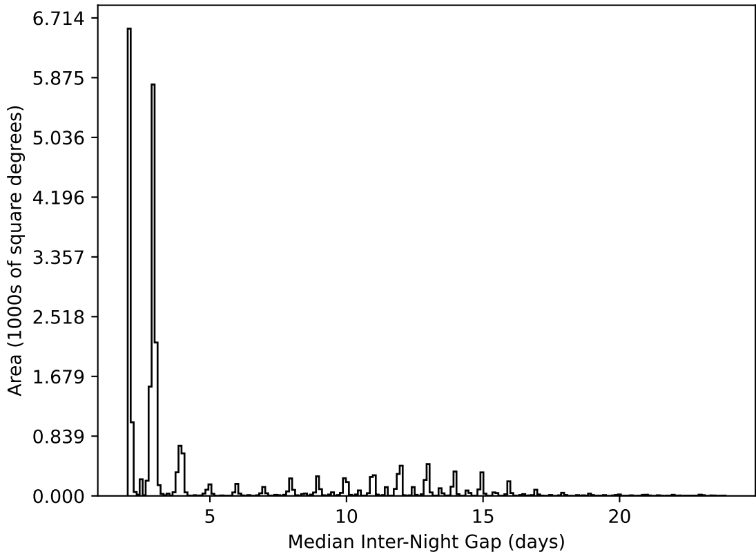
ddf_loaded_fl2_v3.4_10yrs All sky all bands: Median Inter-Night Gap
