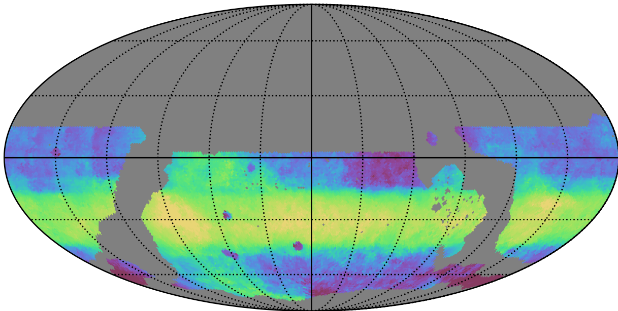
ddf_loaded_fl2_v3.4_10yrs WFD z band: Median HA
