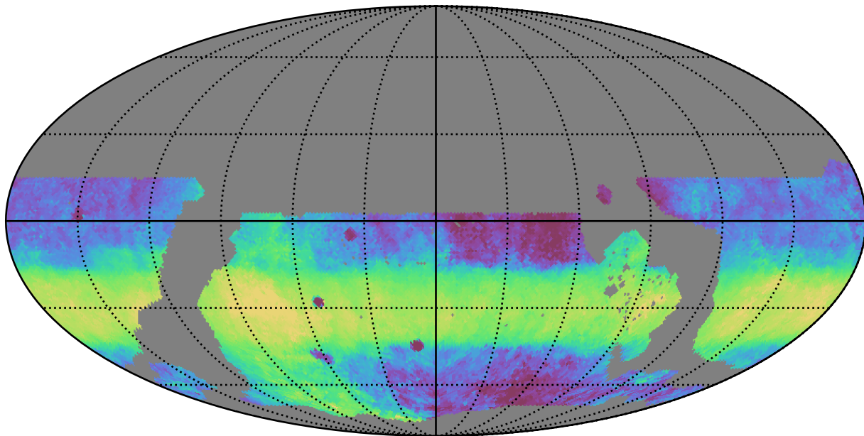
ddf_loaded_fl2_v3.4_10yrs WFD y band: Median HA
