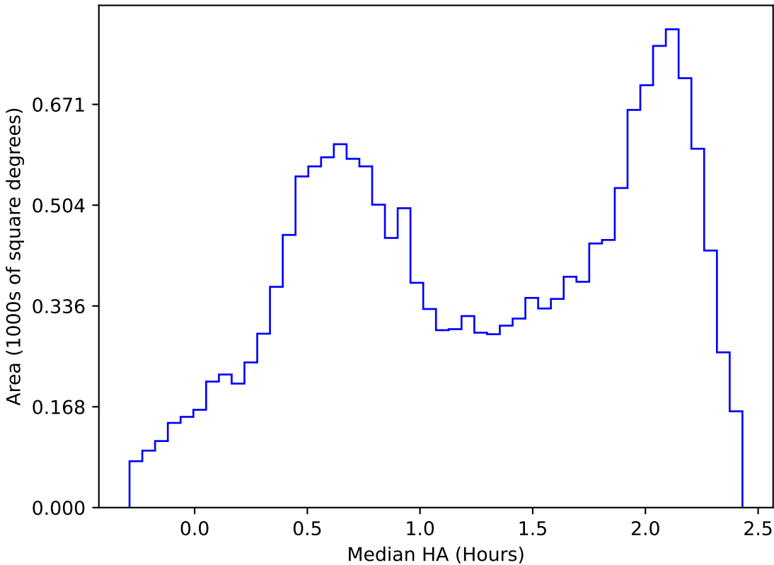
ddf_loaded_fl2_v3.4_10yrs WFD y band: Median HA
