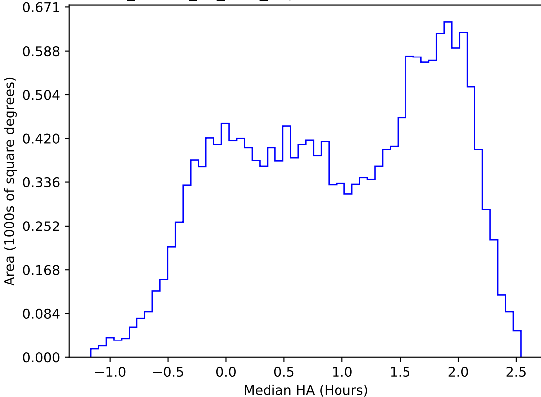
ddf_loaded_fl2_v3.4_10yrs WFD u band: Median HA
