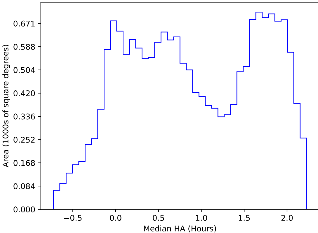
ddf_loaded_fl2_v3.4_10yrs WFD r band: Median HA
