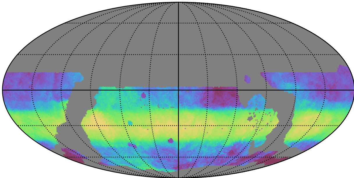
ddf_loaded_fl2_v3.4_10yrs WFD i band: Median HA
