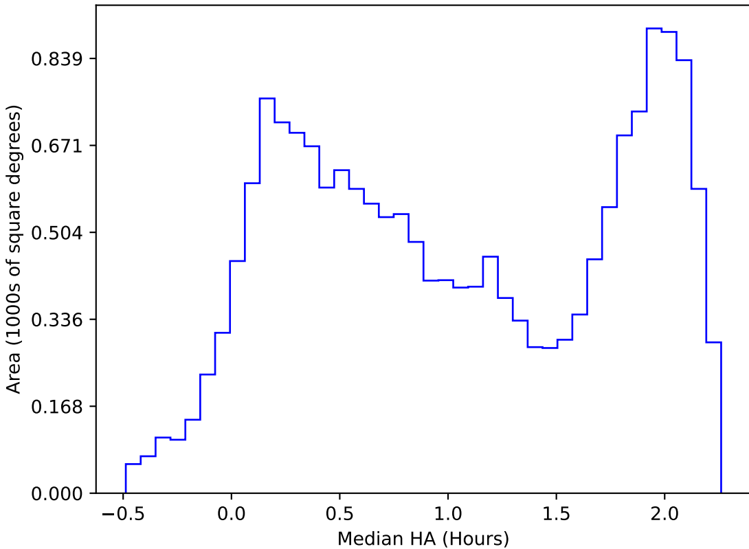
ddf_loaded_fl2_v3.4_10yrs WFD i band: Median HA
