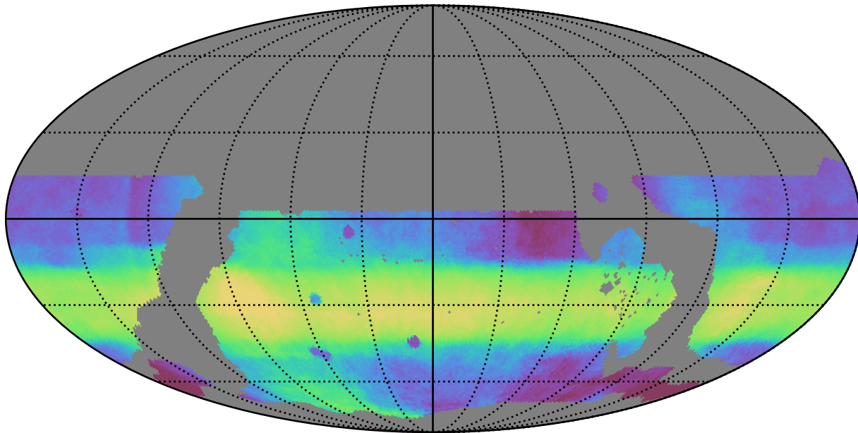
ddf_loaded_fl2_v3.4_10yrs WFD all bands: Median HA
