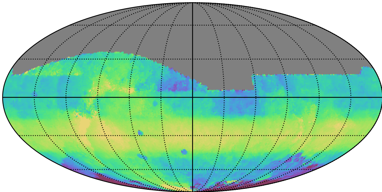
ddf_loaded_fl2_v3.4_10yrs All sky z band: Median HA
