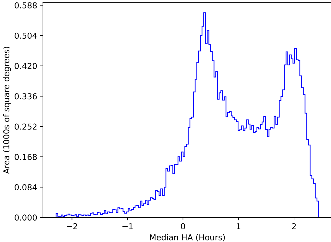
ddf_loaded_fl2_v3.4_10yrs All sky z band: Median HA
