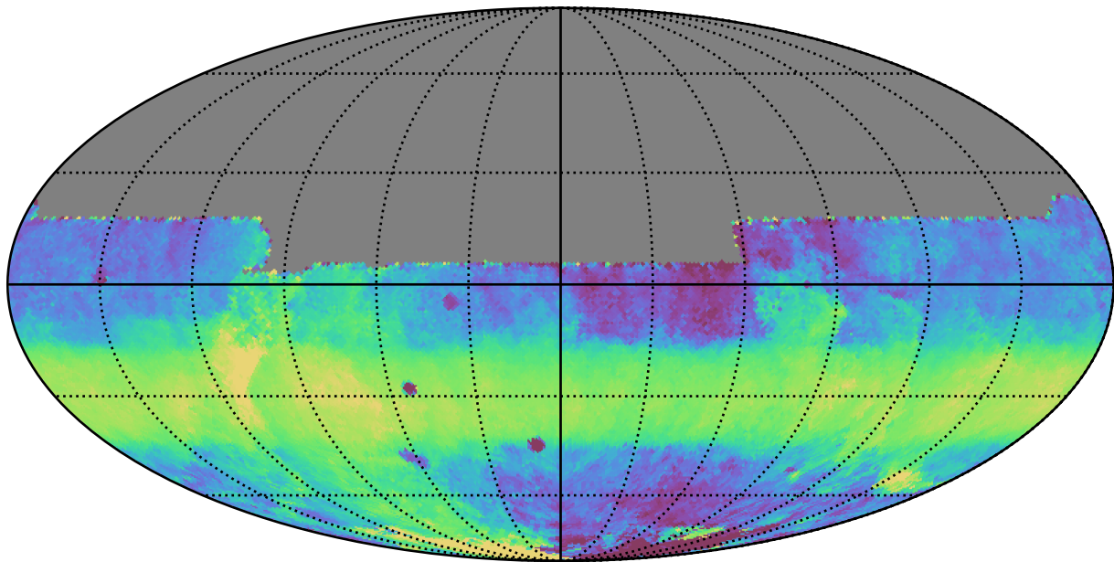
ddf_loaded_fl2_v3.4_10yrs All sky y band: Median HA
