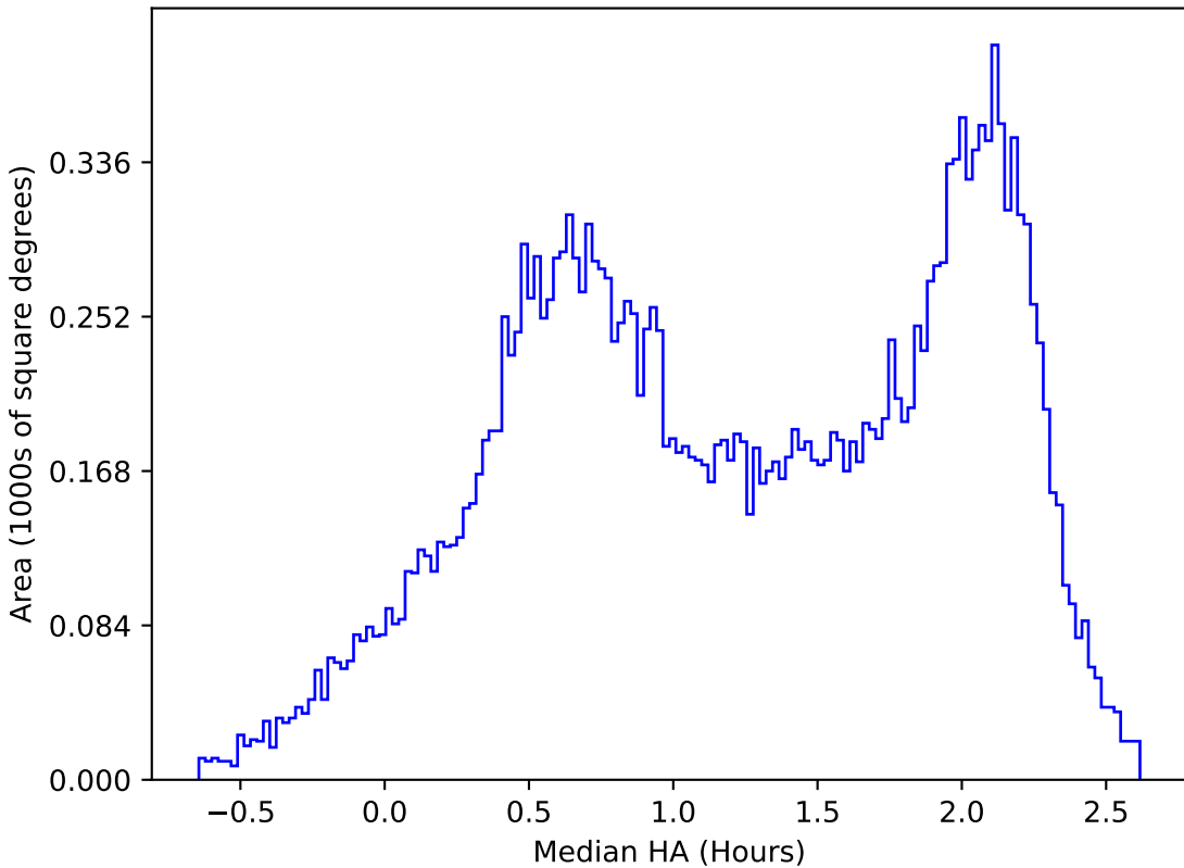
ddf_loaded_fl2_v3.4_10yrs All sky y band: Median HA
