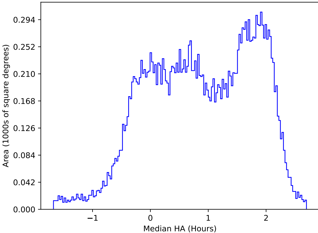
ddf_loaded_fl2_v3.4_10yrs All sky u band: Median HA
