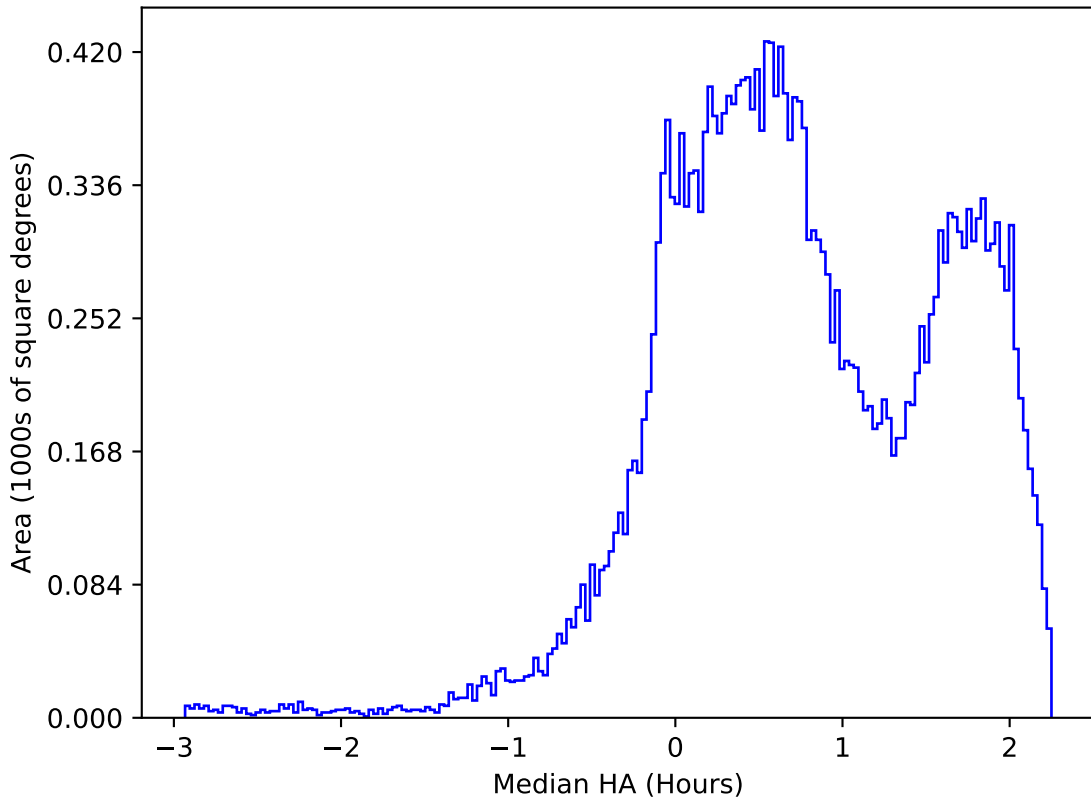
ddf_loaded_fl2_v3.4_10yrs All sky r band: Median HA
