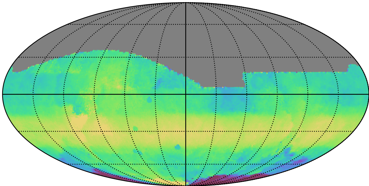
ddf_loaded_fl2_v3.4_10yrs All sky i band: Median HA
